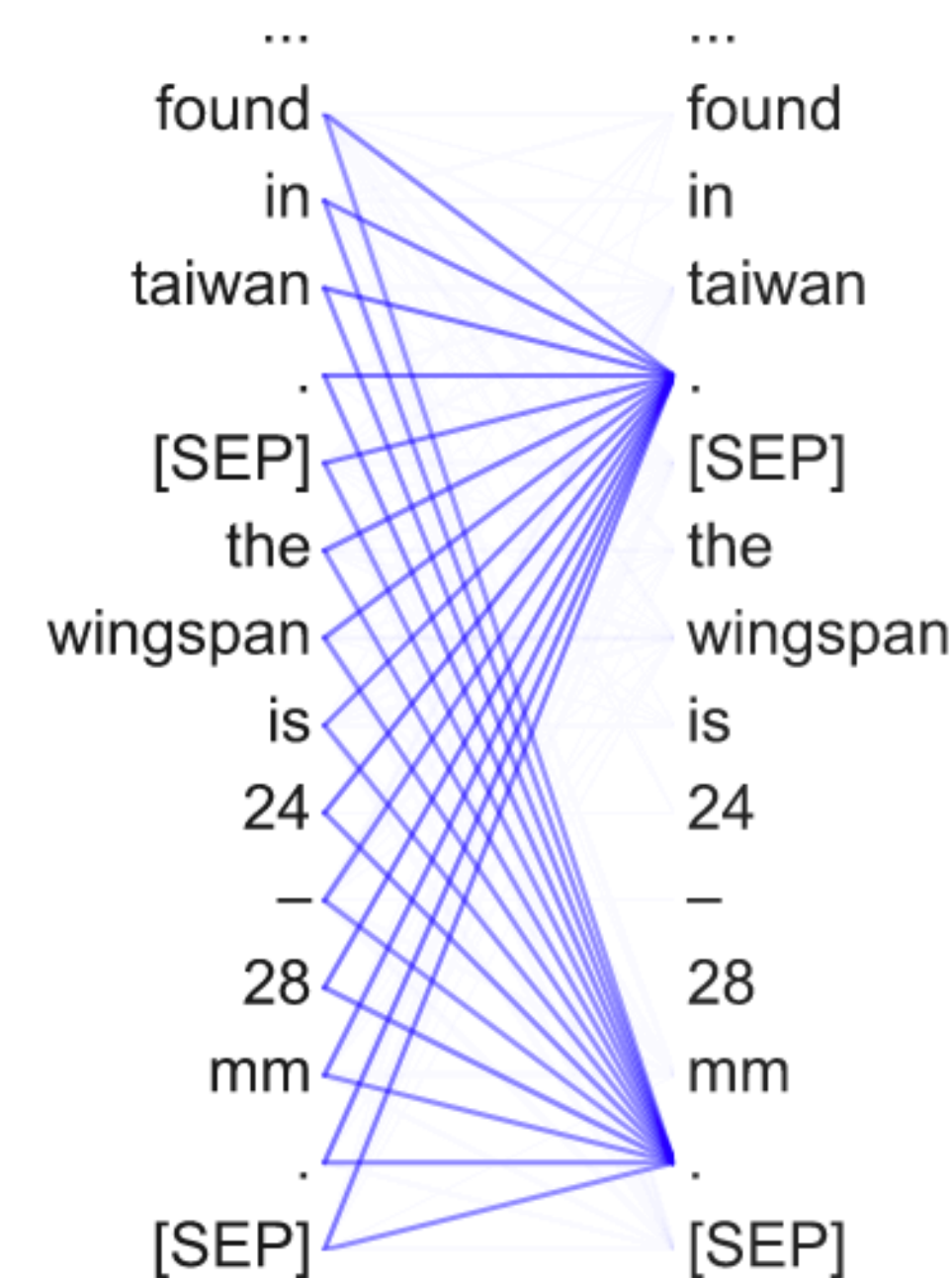
Head 11-6 Attends to periods
