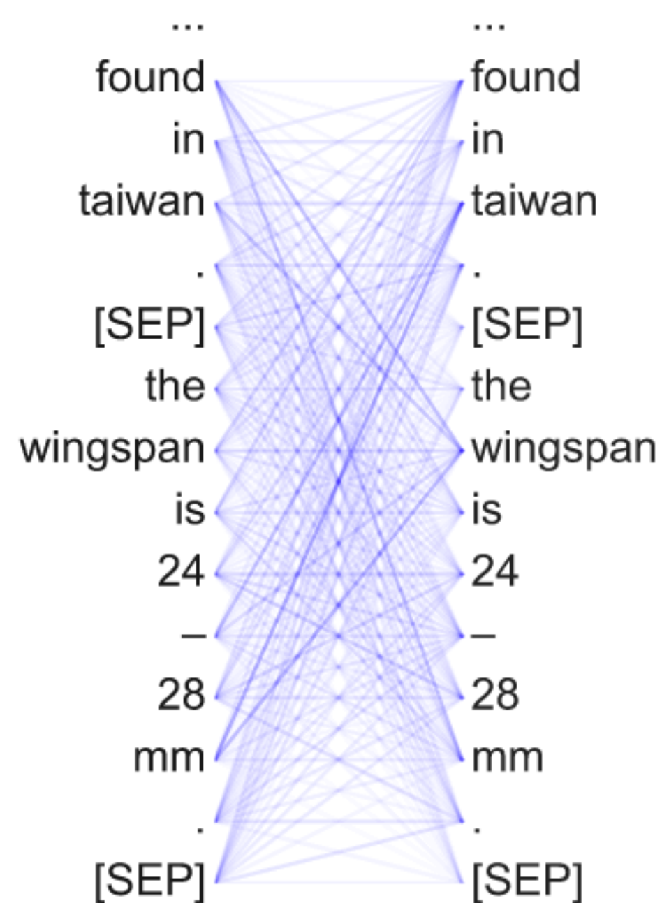
Head 1-1 Attends broadly
