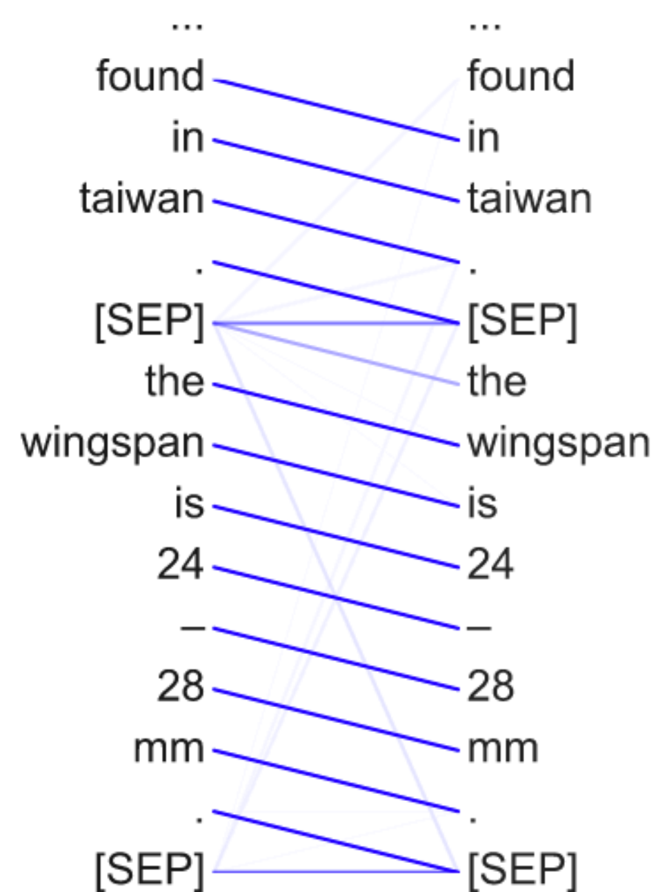
Head 3-1 Attends to next token
