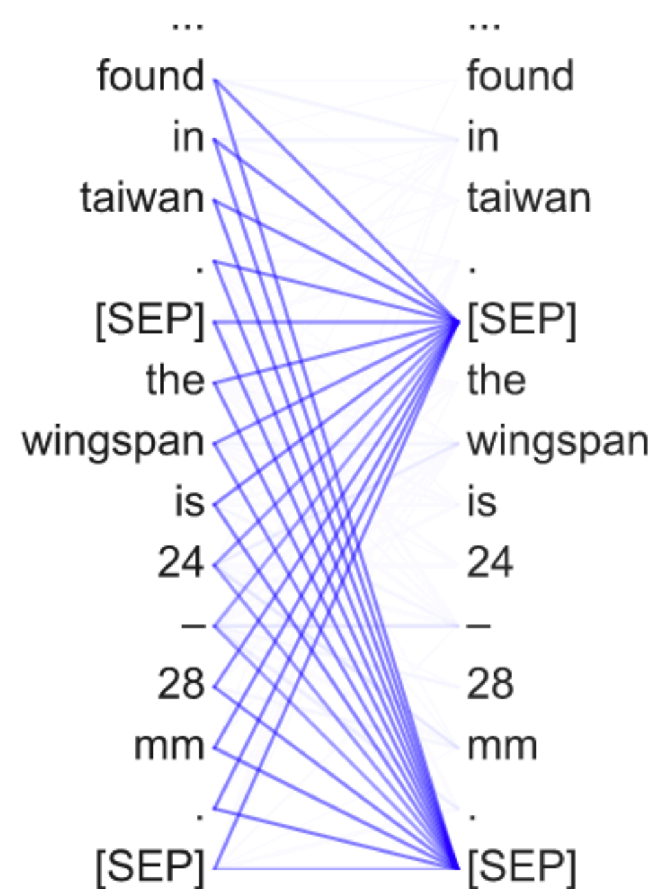
Head 8-7 Attends to [SEP]
